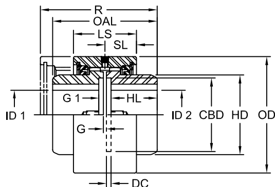
C Type Flex-Flex Coupling
